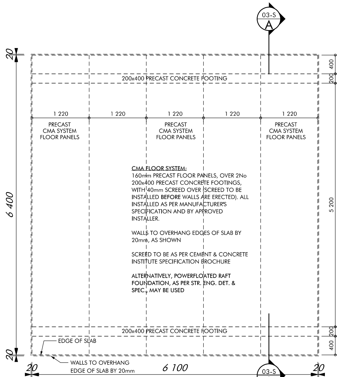
FOUNDATION & SURFACE BED LAYOUT SCALE 1:50
