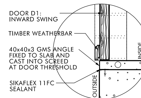
DETAIL 02, SCALE 1:10
