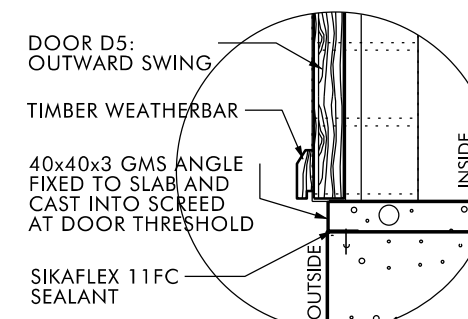
DETAIL 03, SCALE 1:10
