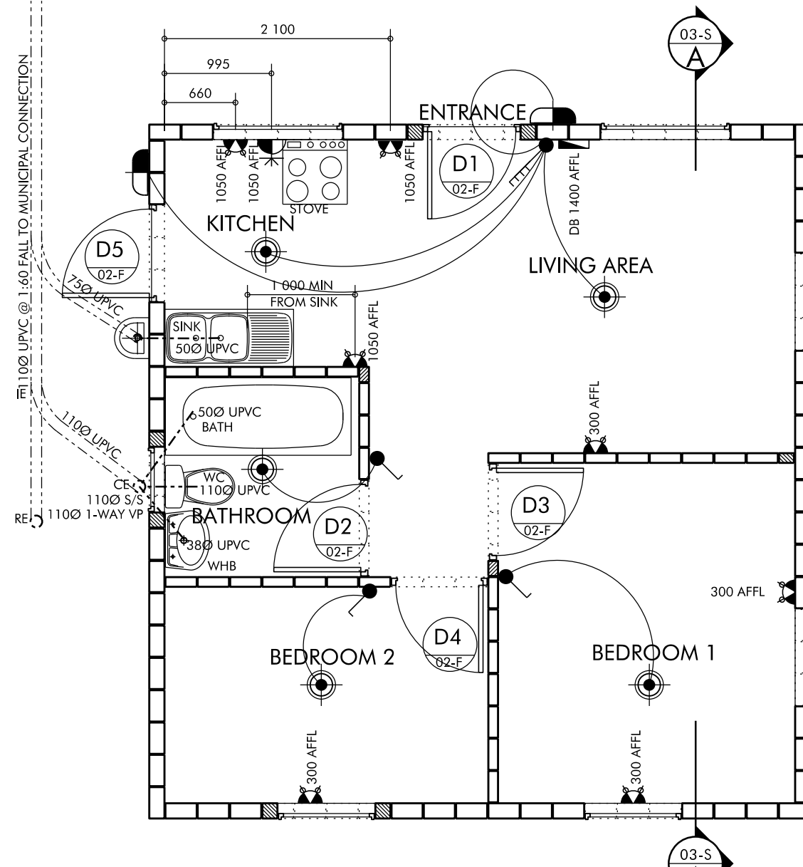
SUGGESTED SERVICES LAYOUT SCALE 1:50
